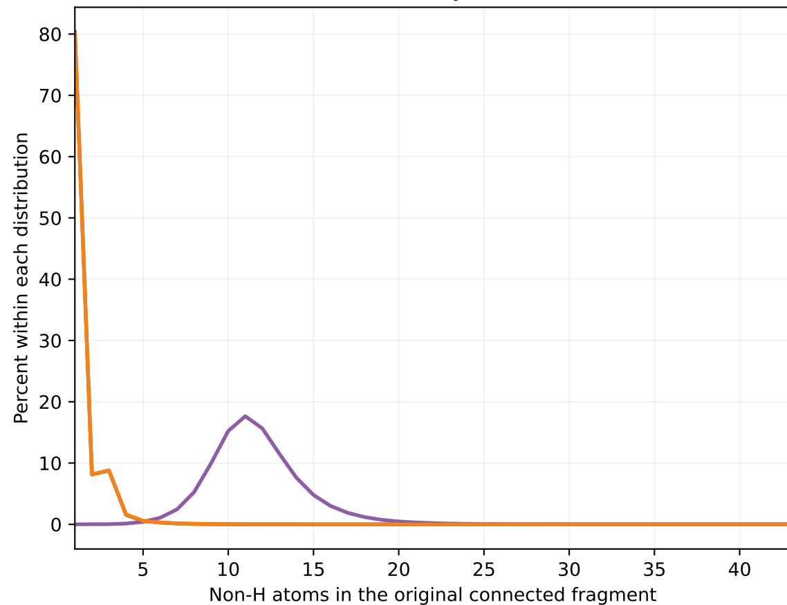
Non-H atom sizes: variety versus occurrences
