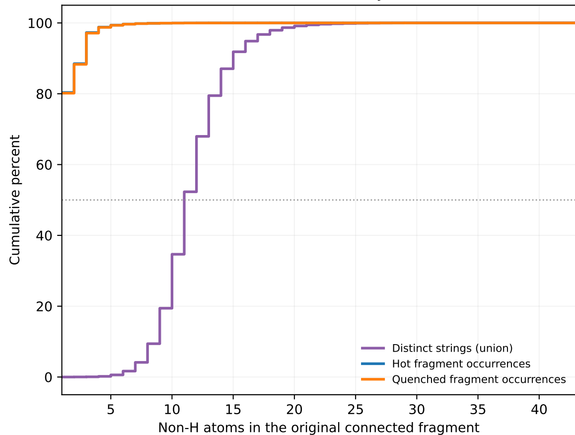
Median: 11 non-H atoms for variety; 1 for occurrences
