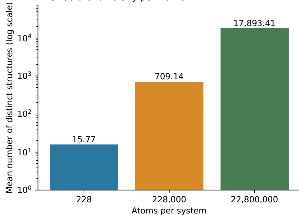
A Structural diversity per frame
