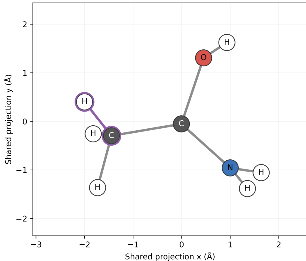
The same ten atom IDs; purple highlights the added C-H connection Before: nine-atom fragment + isolated H After 25 fs: one ten-atom fragment
