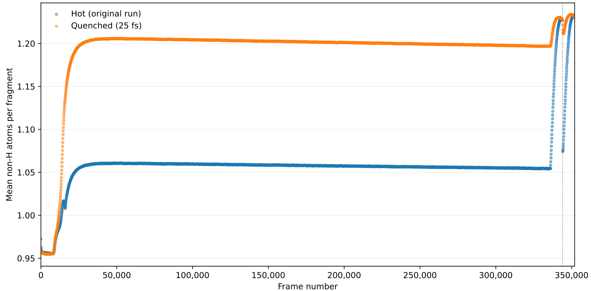
Mean heavy-atom fragment size over the simulation
