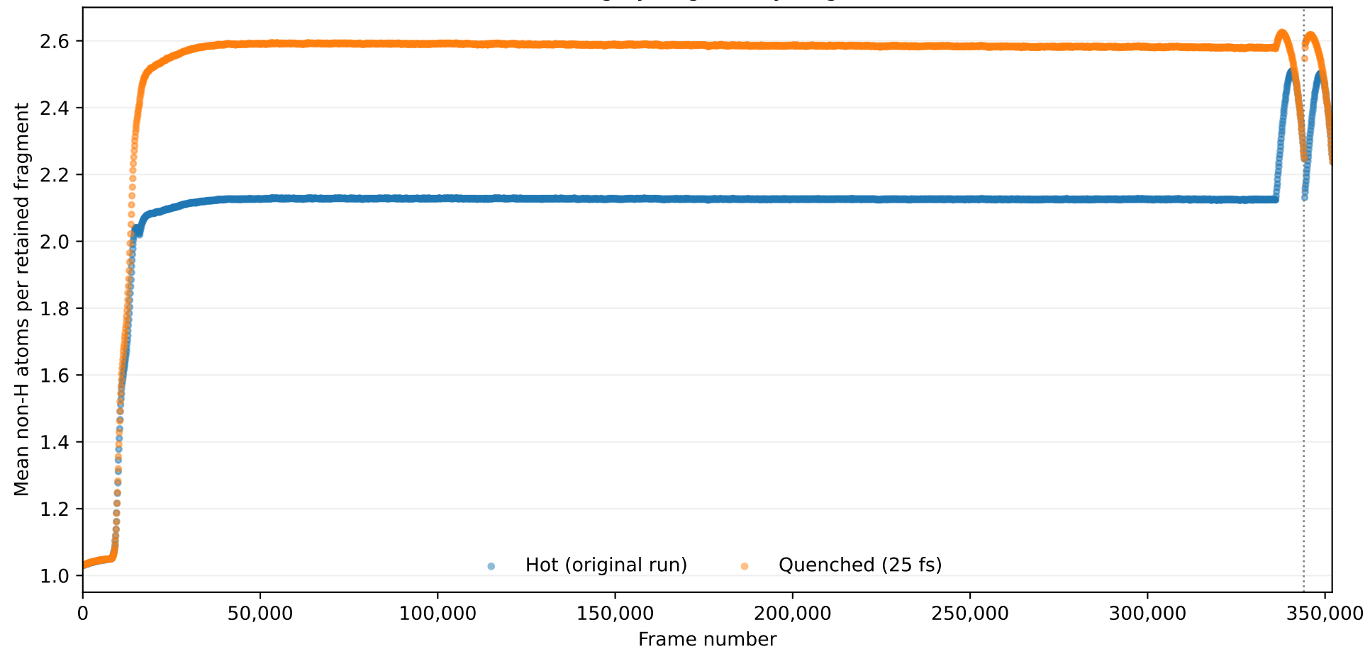
Mean heavy atoms: starting formulas and single atoms excluded Excluding hydrogen-only fragments
