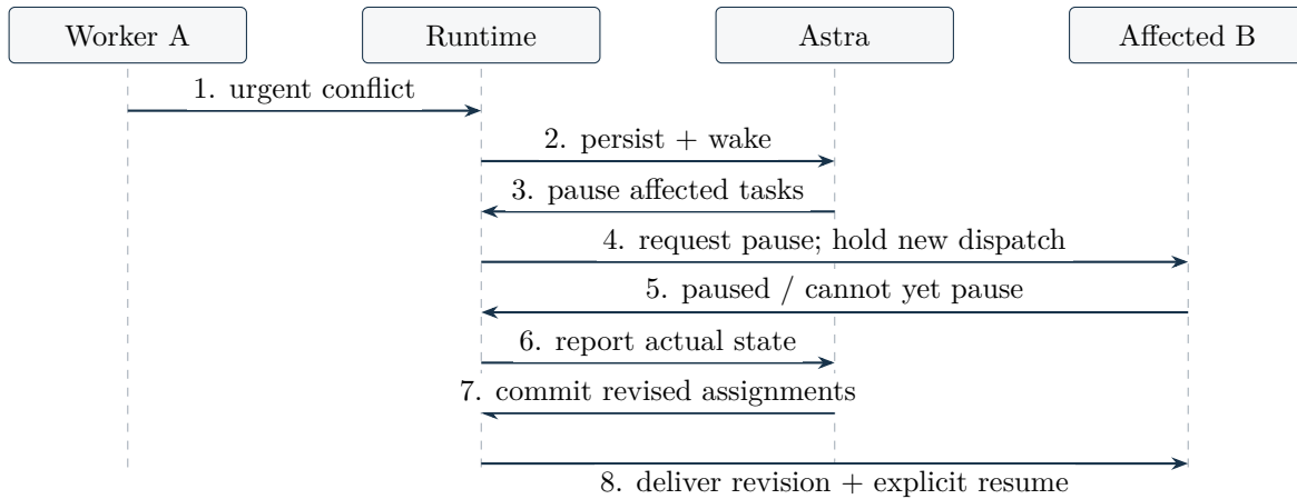
Figure 5. Urgent replan. Worker A stops its own dependent work when blocked. Astra selects affected tasks; unrelated work can continue. A pause is never assumed before confirmation.
