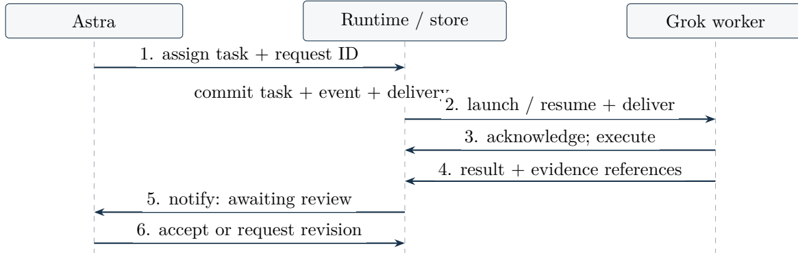
Figure 3. Assignment and result flow. The runtime records Astra’s acceptance decision. Process exit or a zero exit code alone cannot accept a task.
