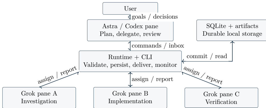
Figure 1. Service relationships. The runtime transports messages; Astra makes coordination decisions. Worker-to-worker messaging is absent by design.
