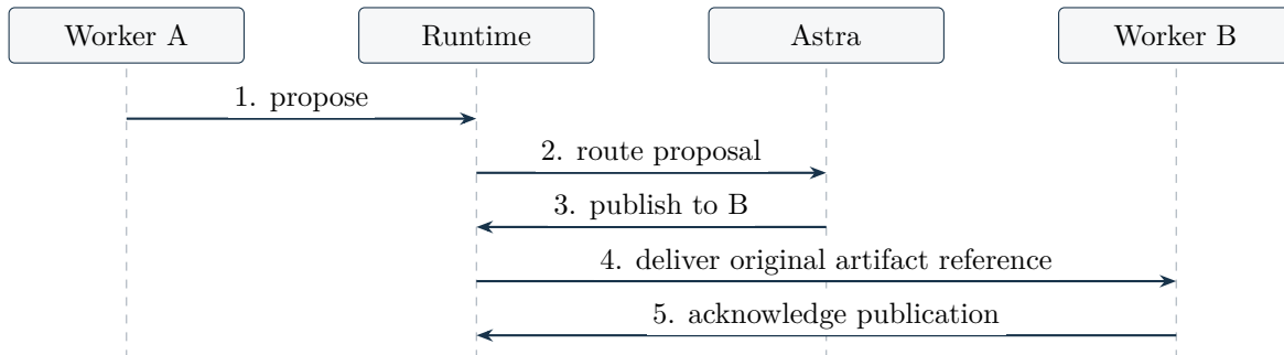
Figure 4. One recipient is shown. Fan-out produces separate delivery records while retaining one publication and its original proposal.
