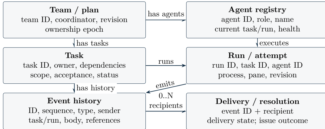
Figure 2. Main record relationships. Event history is immutable; the other records hold current state. All records are scoped to one team.
