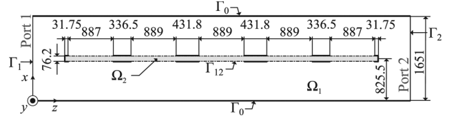
Fig. 1. H-plane cross section of a D-Band passband filter (dielectric slab is shown in light grey; metalization is shown as thick black lines) in a WR6 waveguide. Measures are given in \mu\text{m} .
