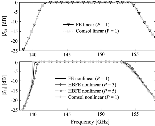
Fig. 2. TE_{10} spectral response for linear (top) and nonlinear (bottom) permittivity with E_i = 10 kV/m. The results are compared with Comsol RF module linear and nonlinear solutions.
