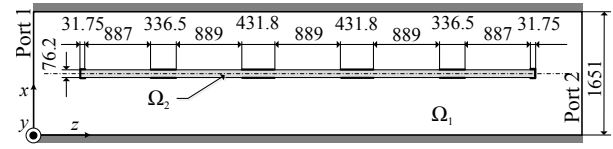
Fig. 2. Cross section (H-plane) of a passband filter realized by placing on the E-plane a dielectric slab partially metalized on both sides (slab is shown in light grey; metal strips - uniform along y are shown as thick black lines) in a WR6 rectangular waveguide. Measures are given in \mu\text{m} .
