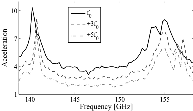
Fig. 5. Acceleration spectrum obtained for a HBFE systems of several harmonic orders. The computations are made for E_i = 10\text{kV/m} .
