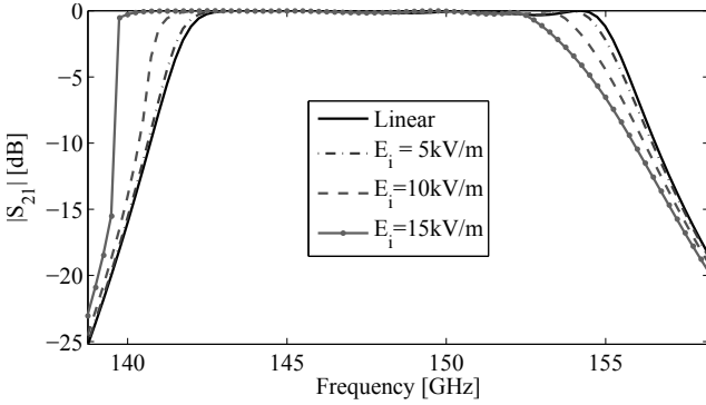
Fig. 4. S_{21} amplitude responses of the nonlinear filter given for several values of E_i compared to the linear case. The field is approximated up to the 5 th harmonic.
