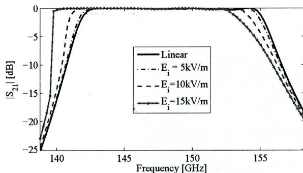
Fig. 4. S_{21} amplitude responses of the nonlinear filter given for several values of E_1 compared to the linear case. The field is approximated up to the 5 th harmonic.
