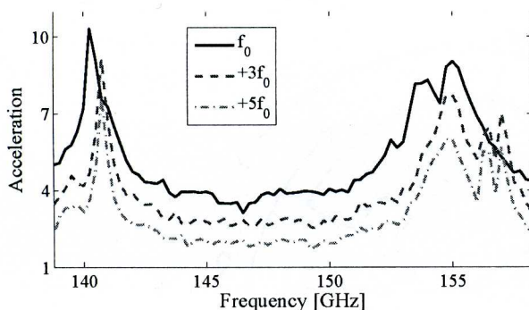
Fig. 5. Acceleration spectrum obtained for a HBFE systems of several harmonic orders. The computations are made for E_1 = 10\text{kV/m} .
