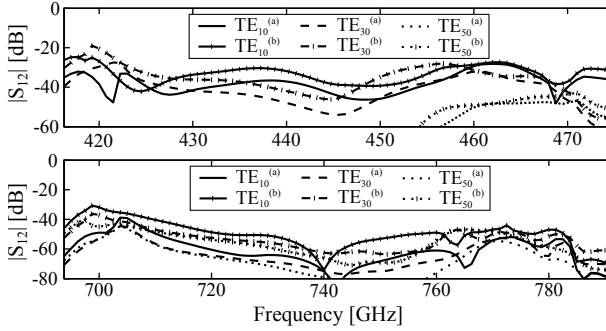
Fig. 5. Spectral responses at 3 rd (top) and 5 th (bottom) harmonics for the relevant guided modes with incident TE_{10} of (a) E_i = 10\text{kV/m} and (b) E_i = 15\text{kV/m} .
