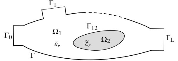
Fig. 1. Generic multiport device where the total domain \Omega is subdivided into a large, linear subdomain \Omega_1 and a smaller subdomain \Omega_2 .
