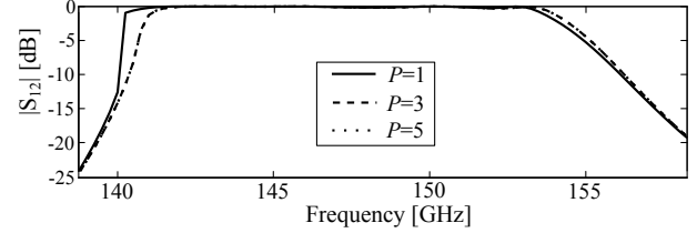
Fig. 3. Behavior of the \text{TE}_{10} spectral response as the number of harmonics retained for the HBFE increases ( E_i = 10\text{kV/m} ).
