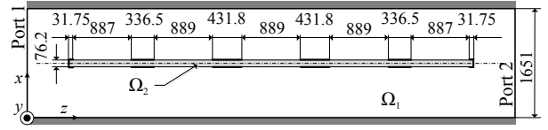
Fig. 2. Cross section (H-plane) of a broadband bandpass filter realized by placing on the E-plane a dielectric slab partially metallized on both sides (slab is shown in light grey; metal strips - uniform along y are shown as thick black lines) in a WR6 rectangular waveguide [14]. Measures are given in \mu\text{m} .
