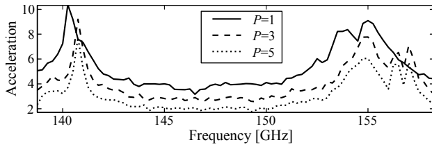
Fig. 6. Acceleration spectrum obtained for a HBFE systems of several harmonic orders. The computations are made for E_i = 10\text{kV/m} .
