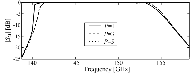
Fig. 3. Behavior of the TE_{10} spectral response as the number of harmonics retained for the HBFE increases ( E_i = 10 \text{ kV/m} ).
