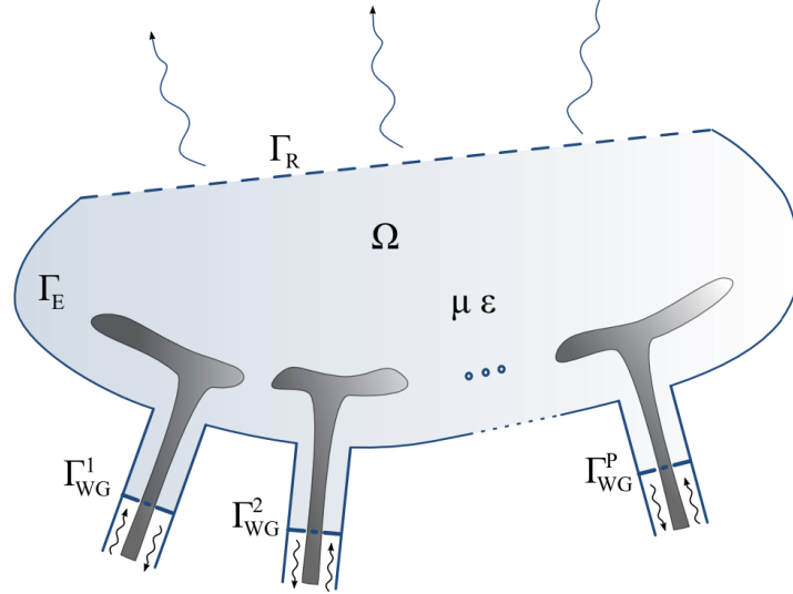
FIG. 1 – Sketch of the phased array antennas finite element analysis domain \Omega .
