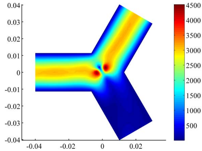
Figure 5. Electric field (V/m) distribution at 10 GHz.
