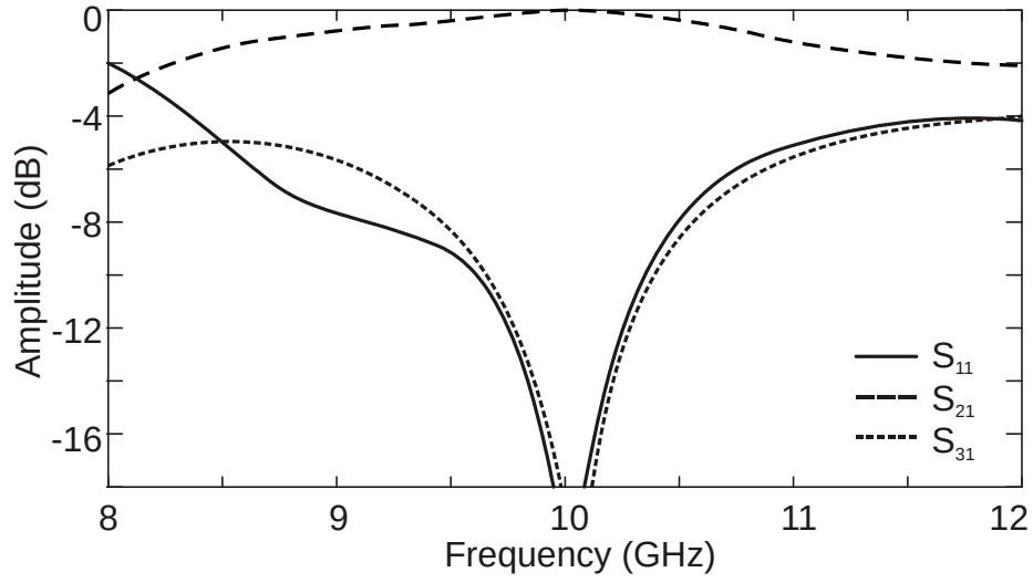
Figure 4. Circulator's small signal frequency response.
