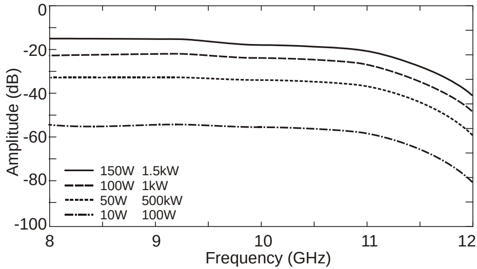
Figure 7. Intermodulation product power at 2f_i - f_s
