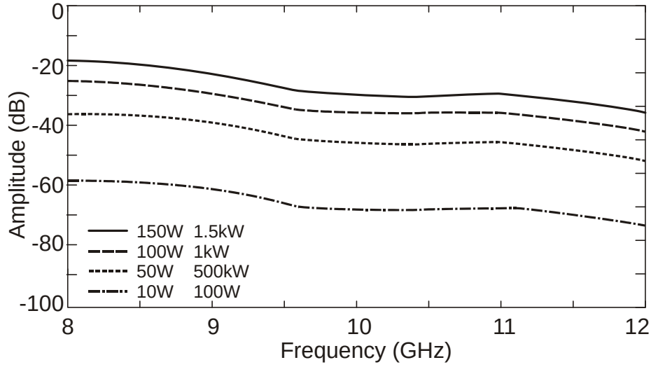
Figure 6. Intermodulation product power at 2f_s - f_i
