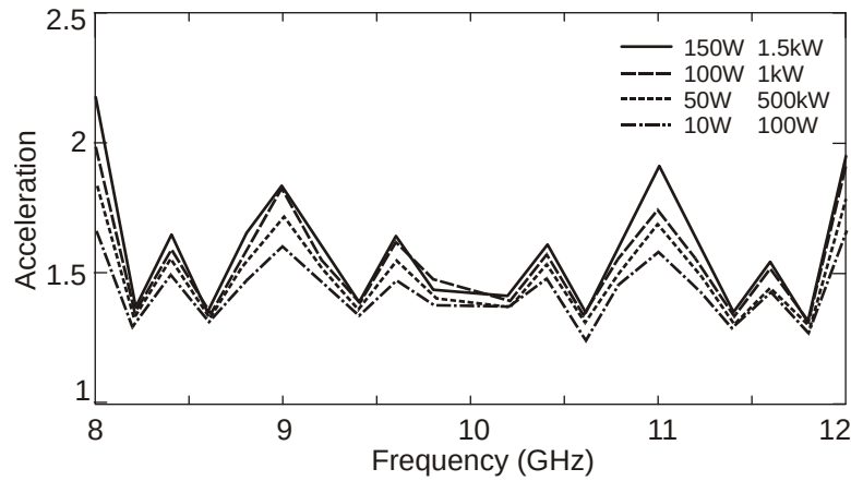
Figure 1. Acceleration of the DD scheme vs conventional scheme.
