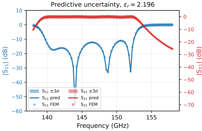
Fig. 8. Overlaid S_{11} and S_{21} predictions at \varepsilon_r = 2.196 (held-out). Solid lines: DKL prediction; markers: FEM ground truth.
