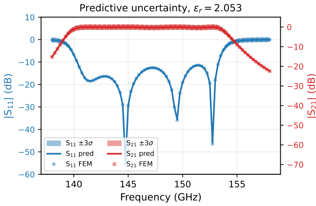
Fig. 7. Overlaid S_{11} and S_{21} predictions at \varepsilon_r = 2.053 (held-out). Solid lines: DKL prediction; markers: FEM ground truth.
