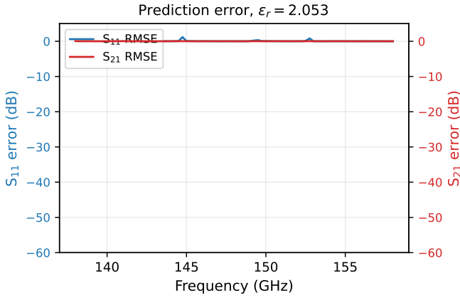
Fig. 7. RMSE curves for S_{11} and S_{21} at \varepsilon_r = 2.053 (held-out). Error: 20 \log_{10}(1 + |S_{\text{pred}} - S_{\text{true}}|/|S_{\text{true}}|) .
