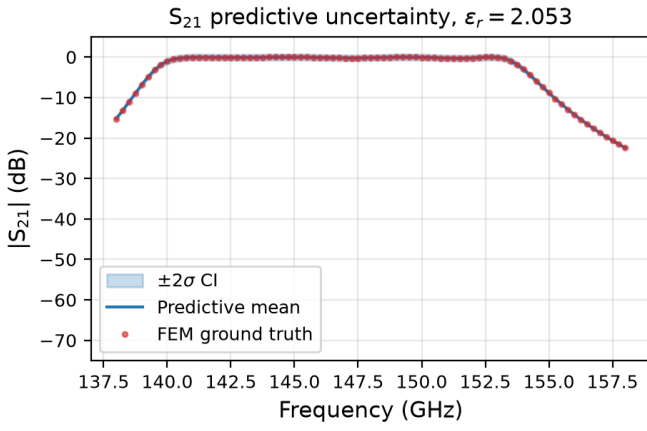
Fig. 7. S_{21} predictive mean and \pm 2\sigma confidence interval for \varepsilon_r = 2.053 (held-out). Shaded: \pm 2\sigma ; dots: FEM ground truth.
