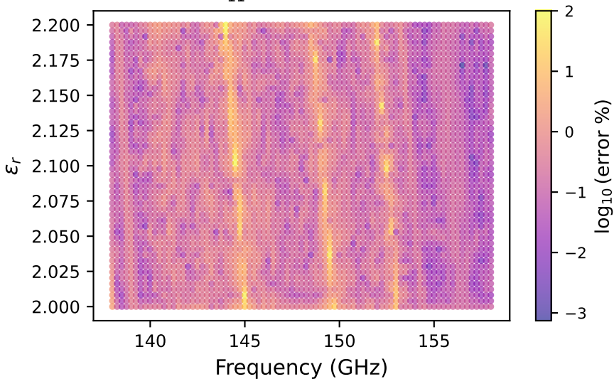
S_{11} relative error
