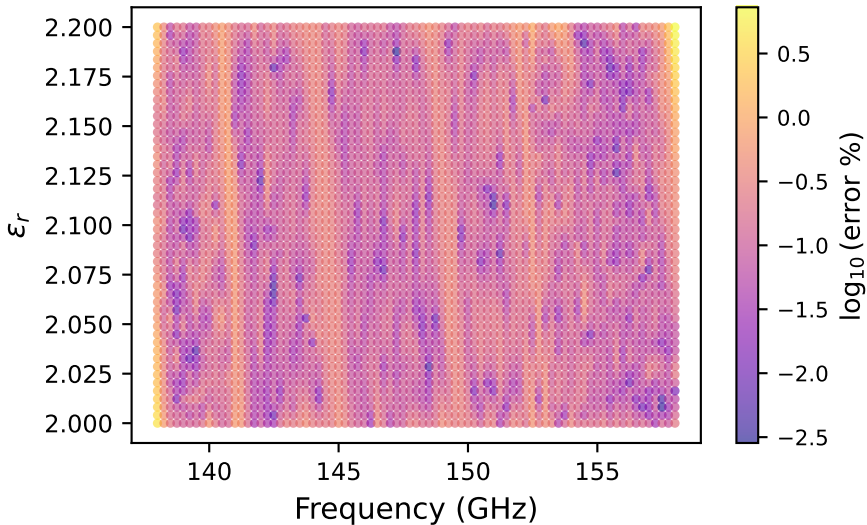
S_{21} relative error
