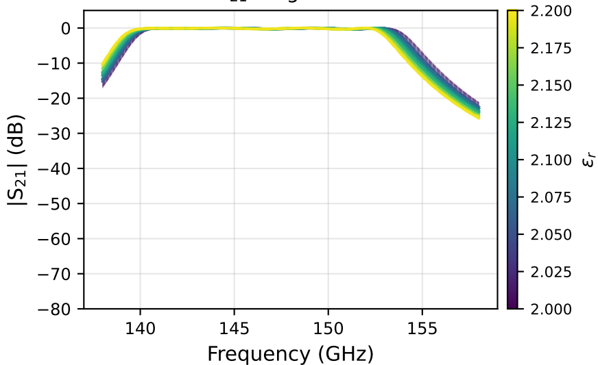
S_{21} magnitude
