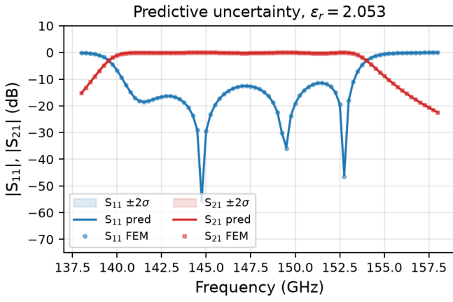
Fig. 7. Predictive mean and \pm 2\sigma confidence interval for S_{11} and S_{21} at \varepsilon_r = 2.053 (held-out). Shaded bands: \pm 2\sigma ; markers: FEM ground truth.
