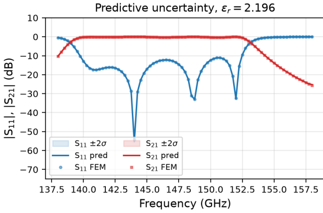
Fig. 8. Predictive mean and \pm 2\sigma confidence interval for S_{11} and S_{21} at \varepsilon_r = 2.196 (held-out). Shaded bands: \pm 2\sigma ; markers: FEM ground truth.
