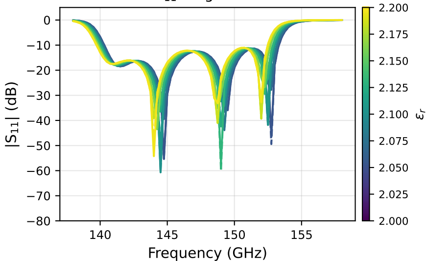
S_{11} magnitude
