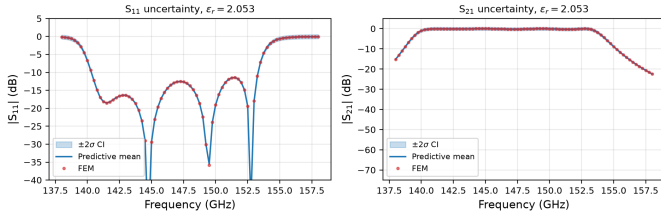
Fig. 7. Predictive mean and \pm 2\sigma confidence interval for \varepsilon_r = 2.053 (held-out). Left: S_{11} ; right: S_{21} . Shaded: \pm 2\sigma ; dots: FEM ground truth.
