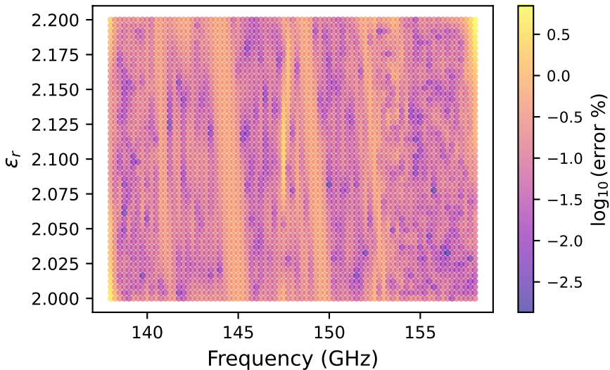
S_{21} relative error
