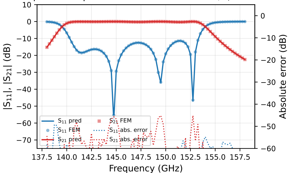
S-parameter predictions and absolute error, \varepsilon_r = 2.053
