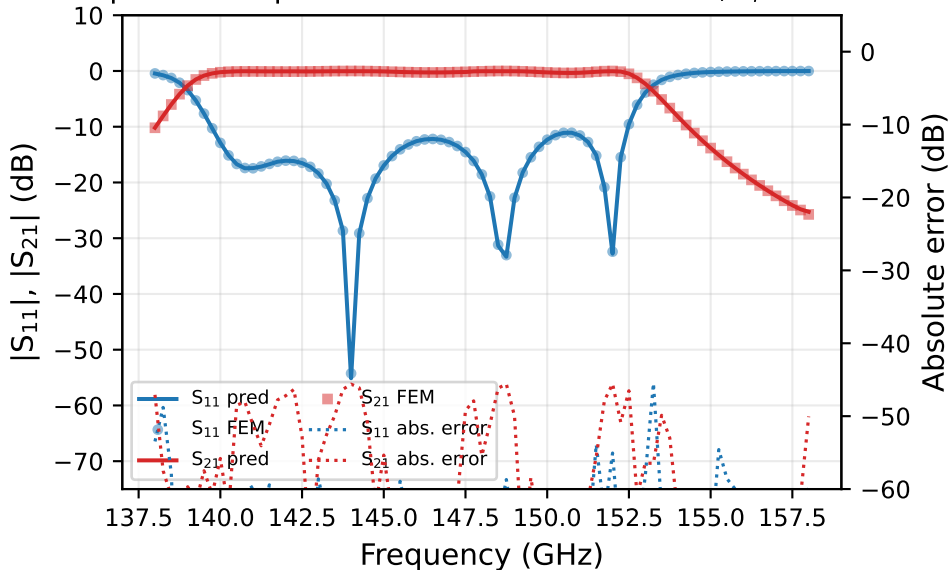
S-parameter predictions and absolute error, \varepsilon_r = 2.196
