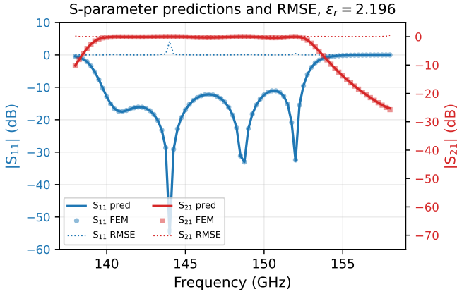
Fig. 8. Predicted and ground truth S_{11} and S_{21} with RMSE curves at \varepsilon_r = 2.196 (held-out).
