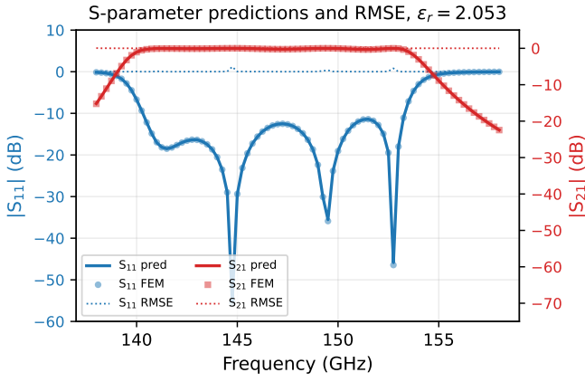
Fig. 7. Predicted and ground truth S_{11} and S_{21} with RMSE curves at \varepsilon_r = 2.053 (held-out). Solid: prediction; markers: FEM; dotted: RMSE.
