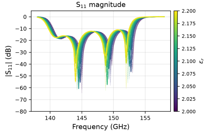
Fig. 1. DKL surrogate reflection magnitude |S_{11}| (dB). Solid: FEM ground truth; dashed: DKL prediction. Bold traces: held-out \varepsilon_r values. Color maps \varepsilon_r \in [2.0, 2.2] .
