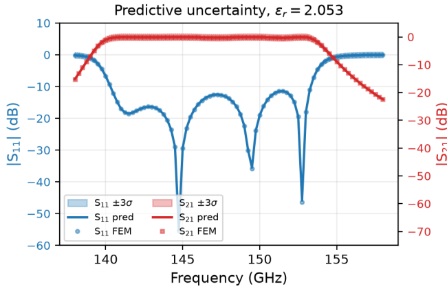
Fig. 7. Predictive mean and \pm 3\sigma confidence interval for S_{11} and S_{21} at \varepsilon_r = 2.053 (held-out). Shaded bands: \pm 3\sigma ; markers: FEM ground truth.
