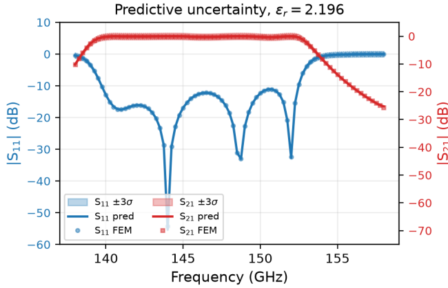
Fig. 8. Predictive mean and \pm 3\sigma confidence interval for S_{11} and S_{21} at \varepsilon_r = 2.196 (held-out). Shaded bands: \pm 3\sigma ; markers: FEM ground truth.
