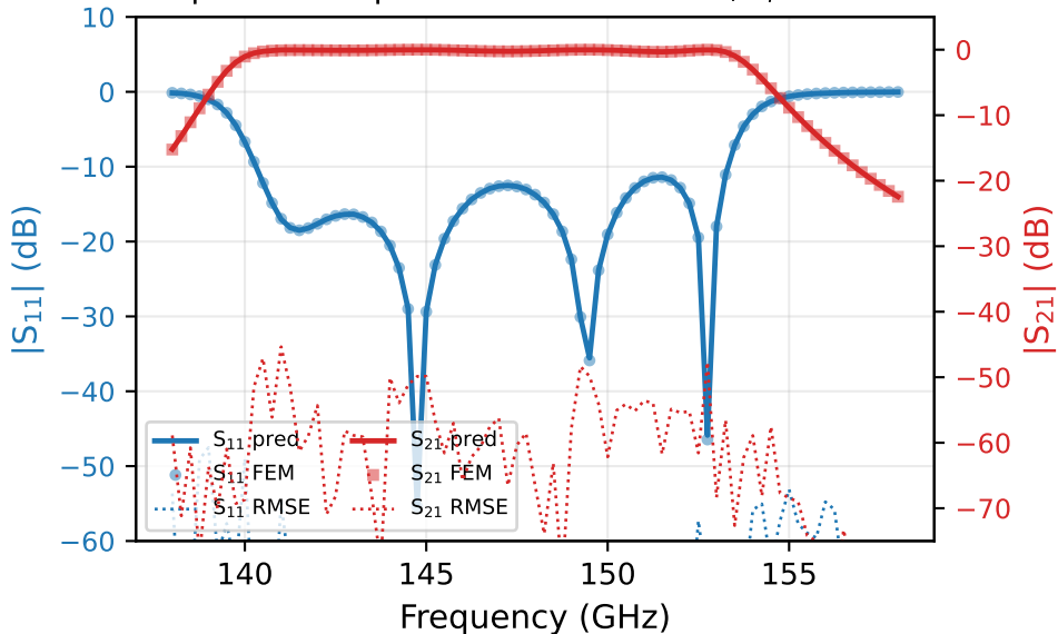
S-parameter predictions and RMSE, \epsilon_r = 2.053
