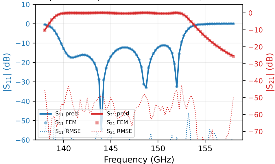
S-parameter predictions and RMSE, \epsilon_r = 2.196
