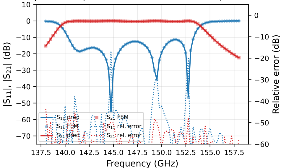
S-parameter predictions and relative error, \varepsilon_r = 2.053
