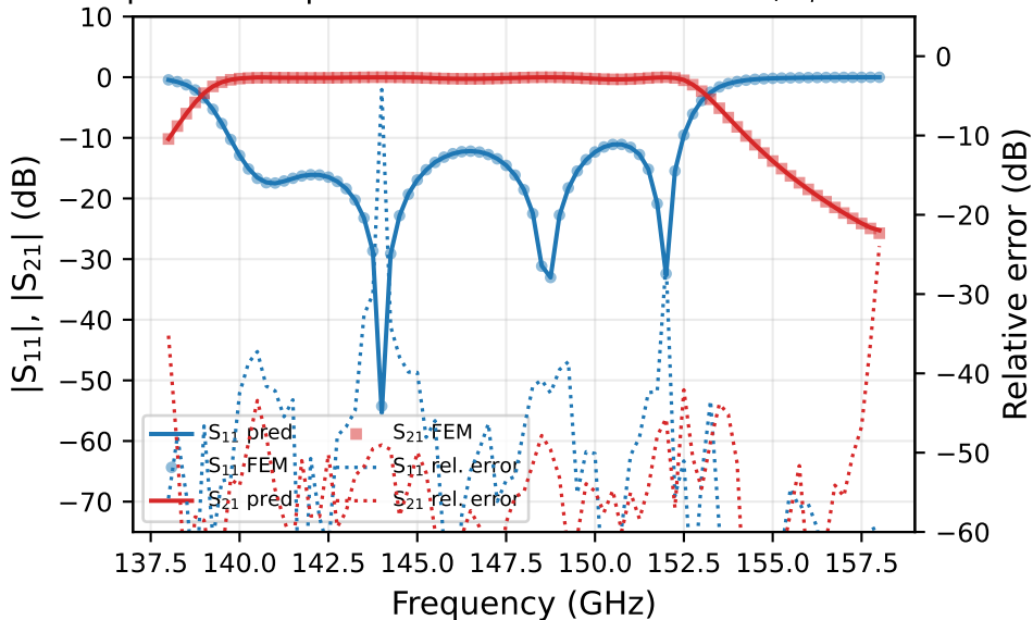
S-parameter predictions and relative error, \varepsilon_r = 2.196
