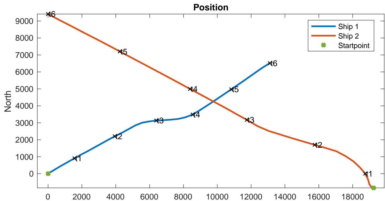
Intention colregs compliant evasive maneuvers
