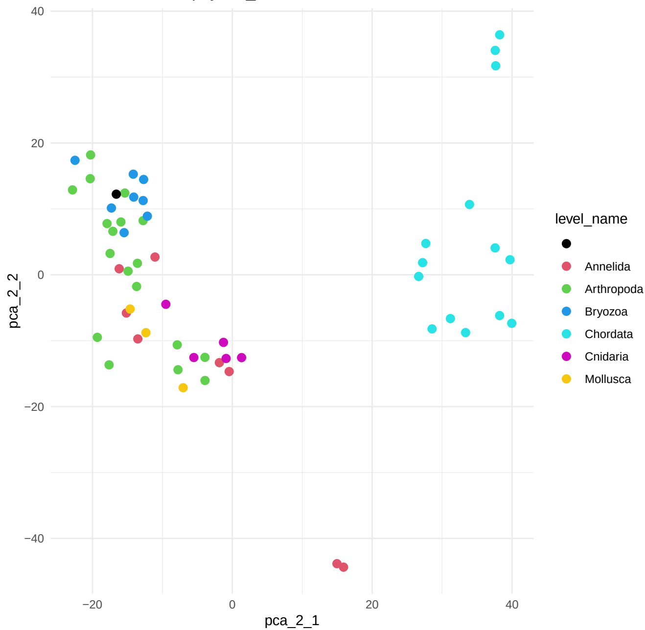
PCA Plot at Level: phylum_name
