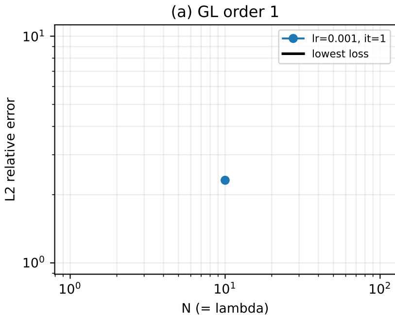
Fig. 4 style: fPINN convergence without FDM curves
