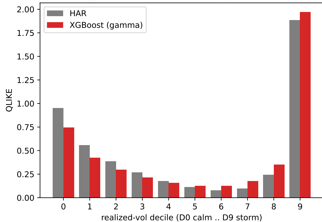
A. h5 per-decile QLIKE (XGBoost (gamma) vs HAR)
