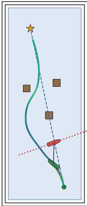
(c) crossing, from port — basin min. range 2.71 m, goal
