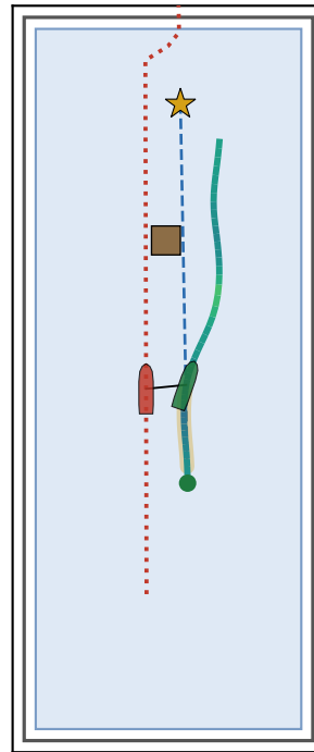
(e) being overtaken — basin min. range 1.40 m, goal
