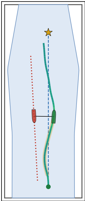
(a) head on — channel min. range 2.56 m, goal
