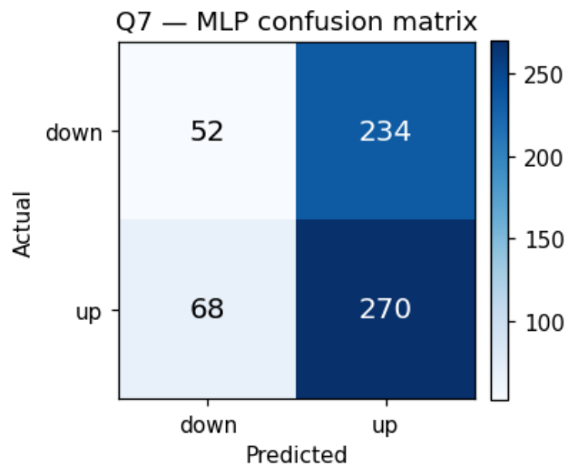
Fig. 7.4 — MLP confusion matrix (test set).
