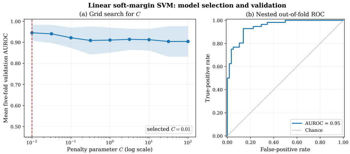
Figure 5: Soft-margin model selection and validation. Panel (a) reports mean five-fold validation AUROC with one standard deviation across folds for every candidate C ; the dashed line marks the selected value. Panel (b) reports the nested out-of-fold ROC obtained when C is selected inside each outer training fold.
