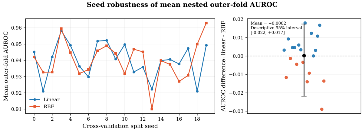
Figure 14: Seed-robustness of the fairer mean outer-fold AUROC. Panel (a): linear and RBF values across twenty fold-assignment seeds. Panel (b): the per-seed difference (linear minus RBF) with its mean and descriptive 95% interval. The interval straddles zero, showing that neither model has a stable within-fold discrimination advantage across splits.
