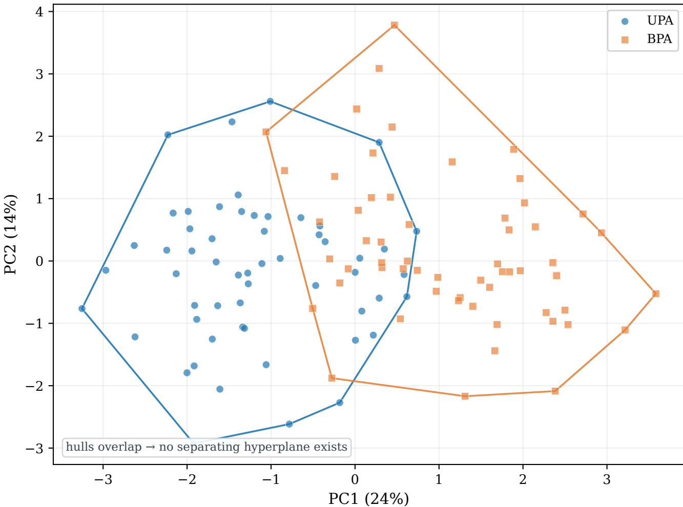
Overlapping convex hulls of the two subtypes (PC1/PC2)
