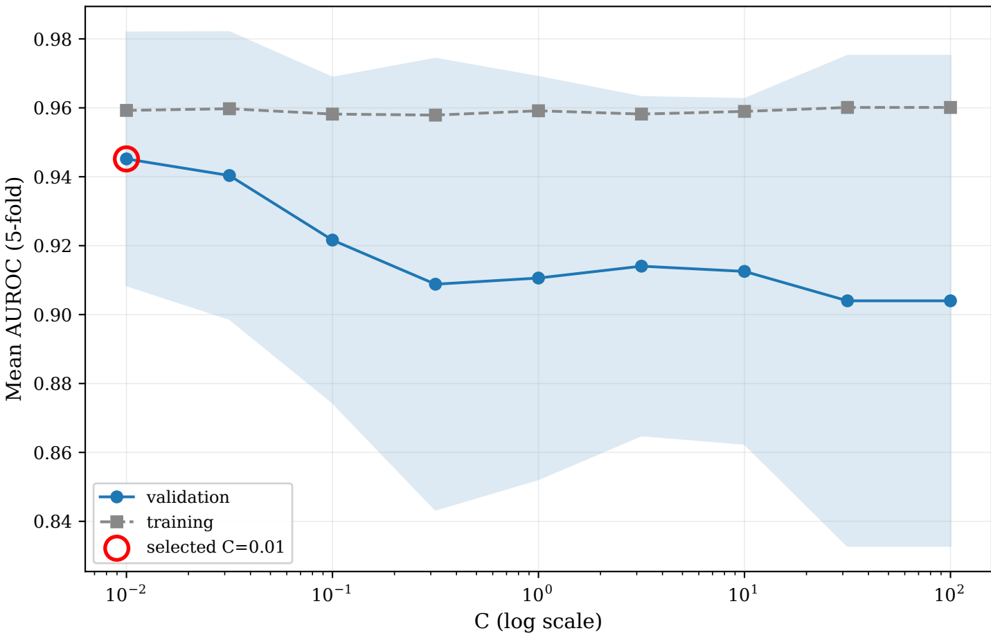
Soft-margin grid search for C
