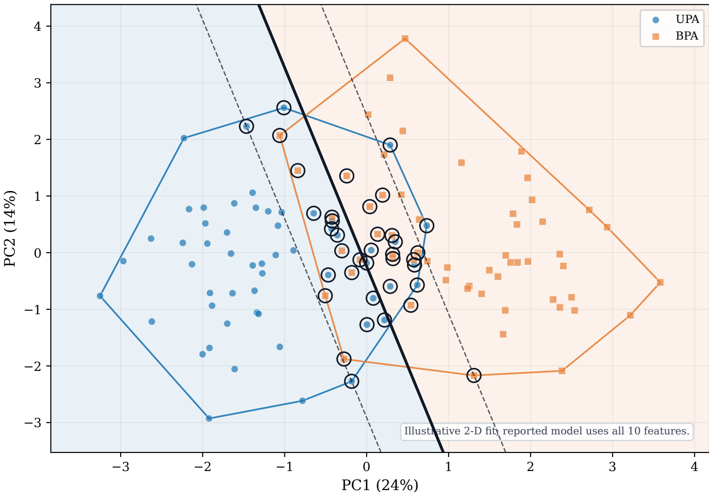
Soft-margin linear boundary in PC1/PC2
