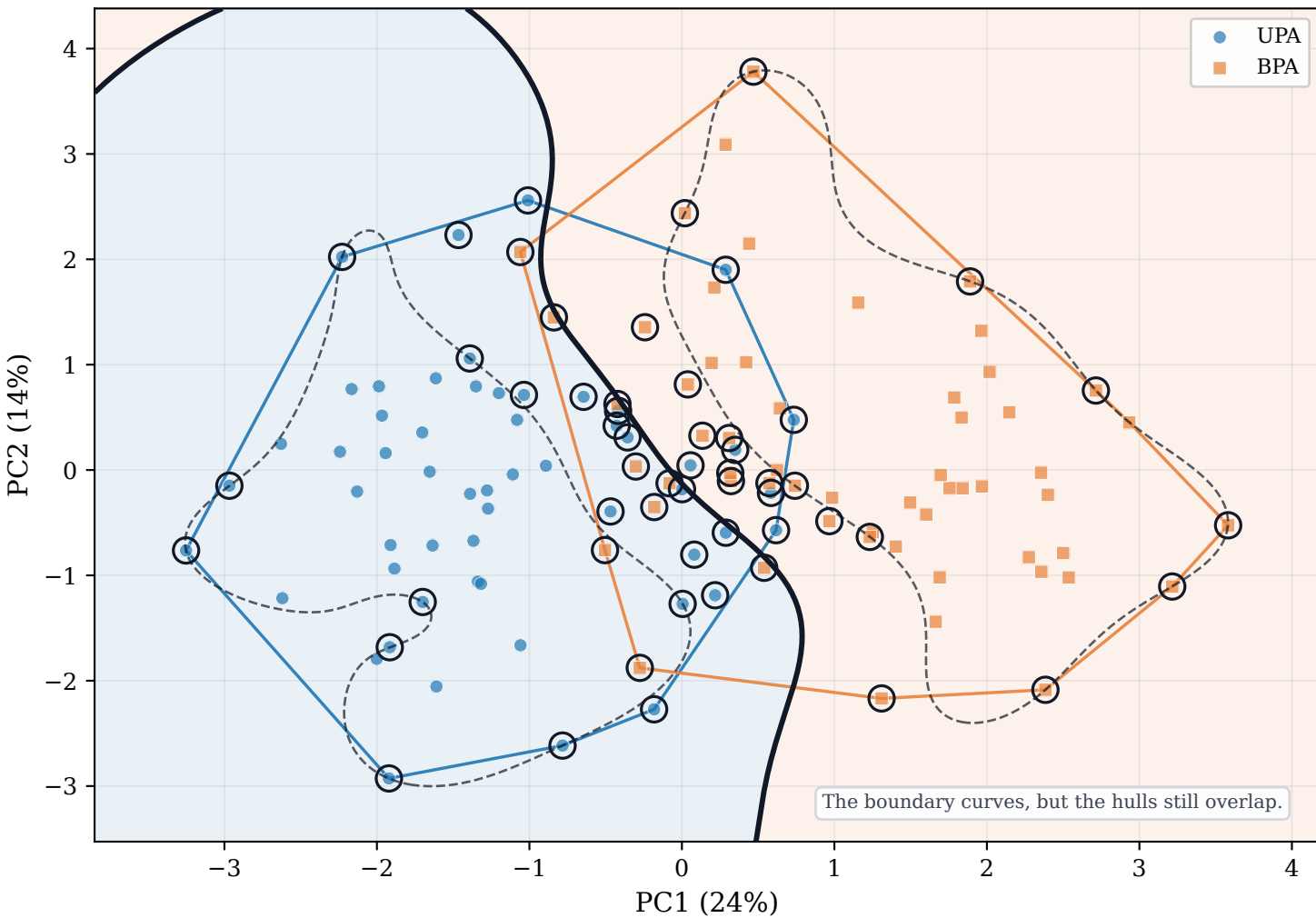
RBF-kernel boundary in the same PC1/PC2 space
