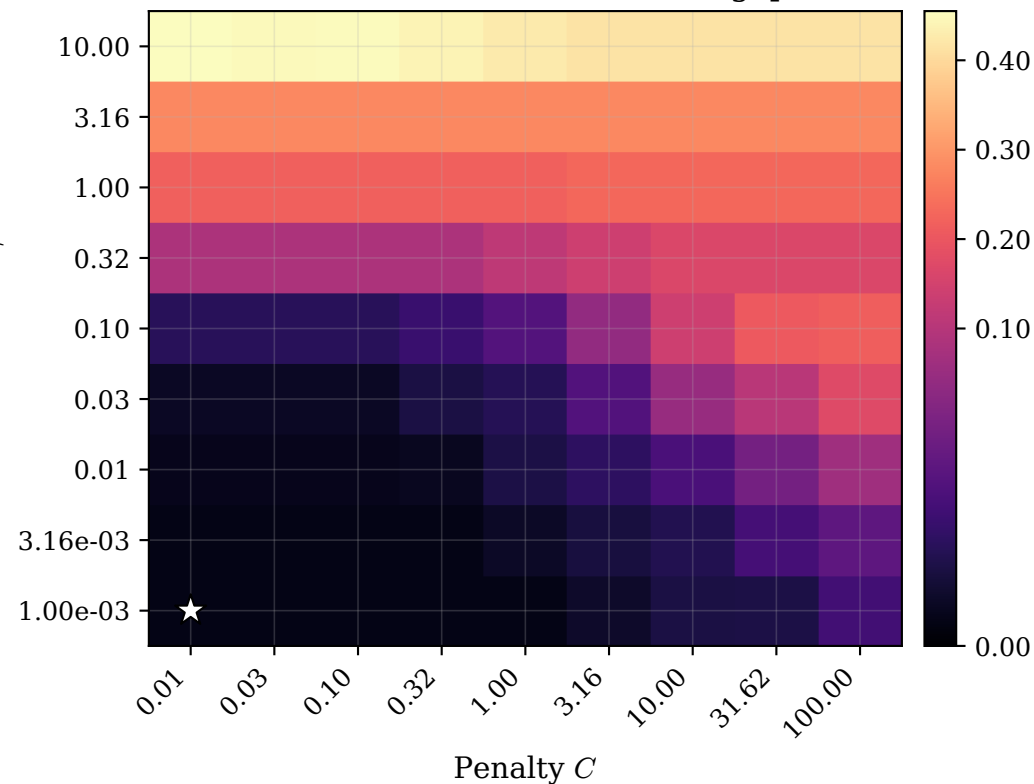
(b) Train--validation AUROC gap
