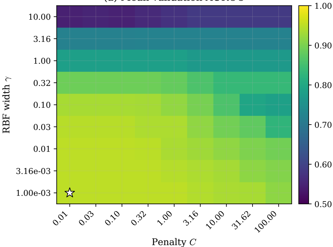
(a) Mean validation AUROC
