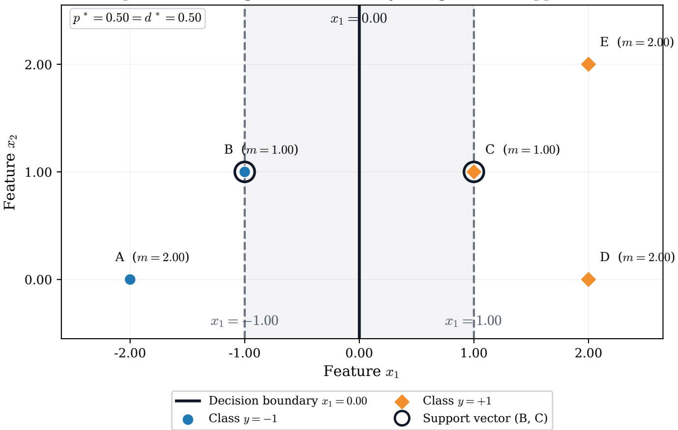
Five-point hard-margin SVM: boundary, margins, and support vectors
