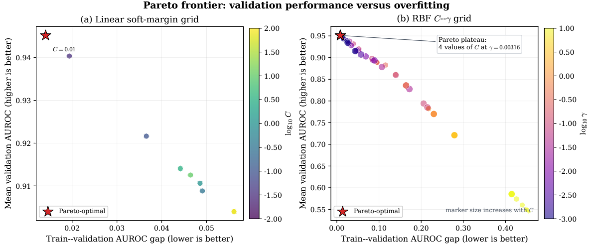
Figure 7: Pareto analysis of the linear and RBF tuning grids. The horizontal axis is the train-validation AUROC gap, so smaller values are preferred; the vertical axis is mean validation AUROC, so larger values are preferred. Red stars mark non-dominated settings. In panel (a), color represents \log_{10} C . In panel (b), color represents \log_{10} \gamma and marker size increases with C .
