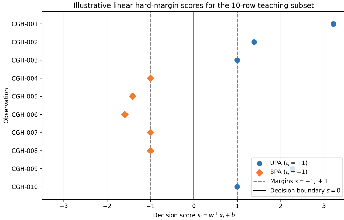
Figure 5: Decision scores for the separable ten-row teaching subsystem. This is an algebraic illustration, not a validation or ROC result.
