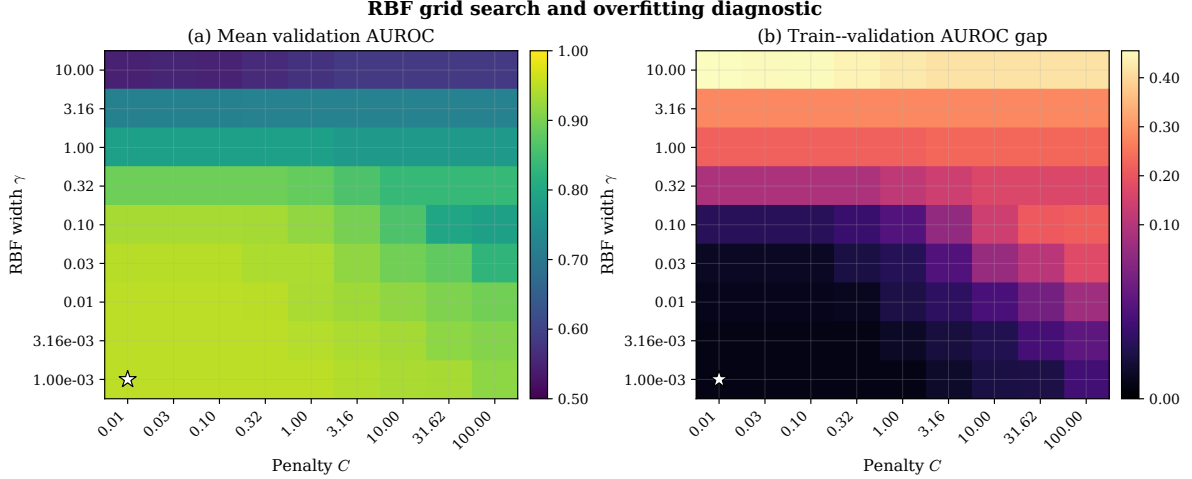
Figure 6: Joint RBF grid search. Panel (a) shows mean validation AUROC. Panel (b) shows mean training AUROC minus mean validation AUROC; large positive values indicate overfitting. The white star marks the selected full-data pair C = 0.01 , \gamma = 1.00 \times 10^{-3} .
