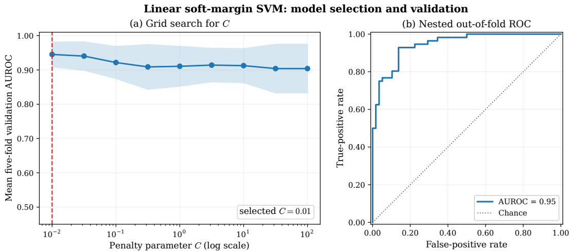
Figure 3: Soft-margin model selection and validation. Panel (a) reports mean five-fold validation AUROC with one standard deviation across folds for every candidate C ; the dashed line marks the selected value. Panel (b) reports the nested out-of-fold ROC obtained when C is selected inside each outer training fold.
