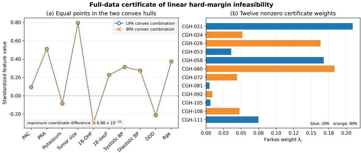
Figure 4: Full-data infeasibility certificate. Panel (a) shows the identical ten-dimensional point obtained as a convex combination of UPA observations and as a convex combination of BPA observations; the plot compares coordinates directly and is not a two-dimensional projection. Panel (b) shows the twelve nonzero Farkas weights.
