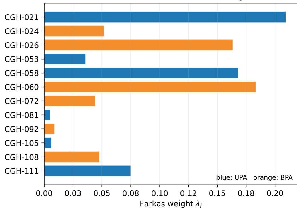
(b) Twelve nonzero certificate weights
