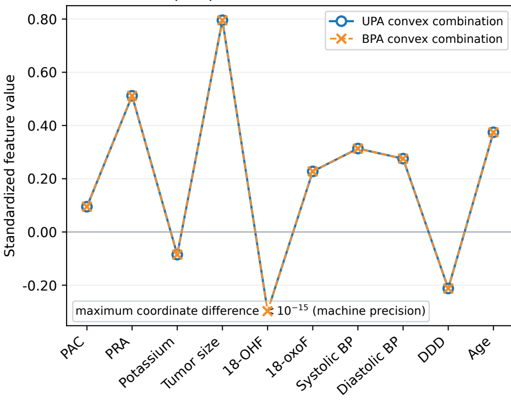
(a) Equal points in the two convex hulls
