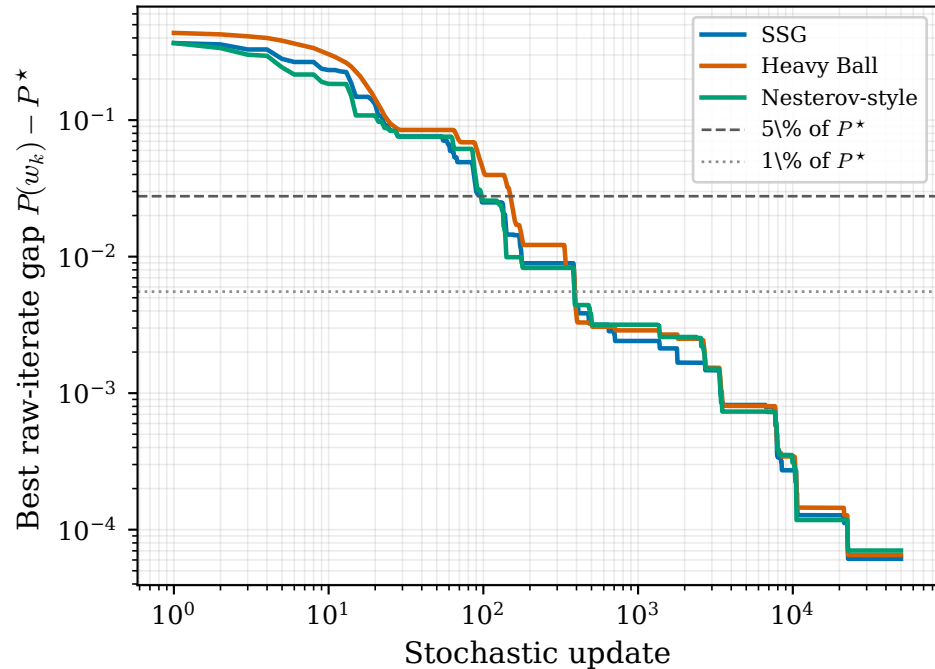
Best objective gap
