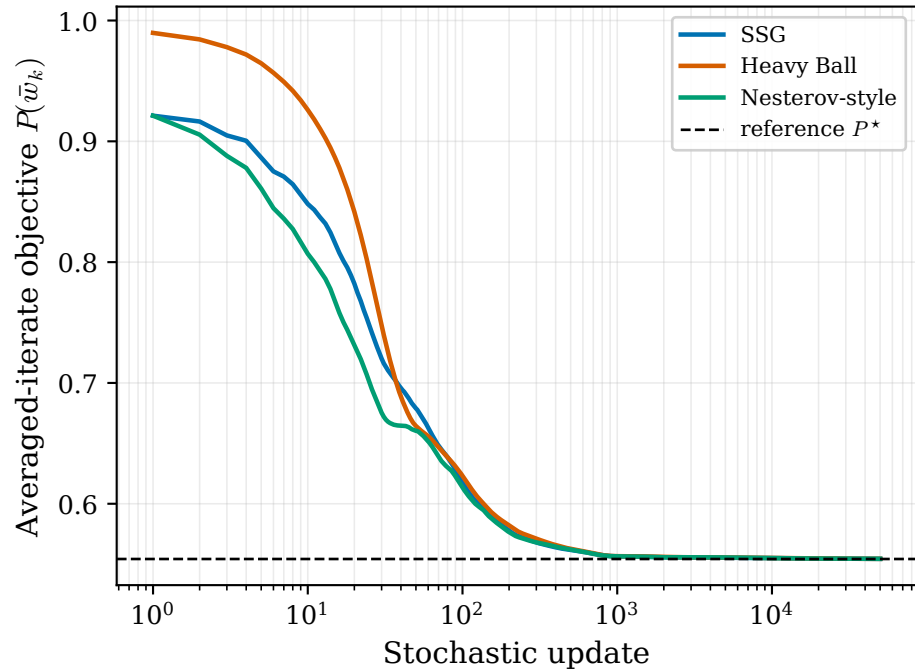
Objective convergence at C=0.01
