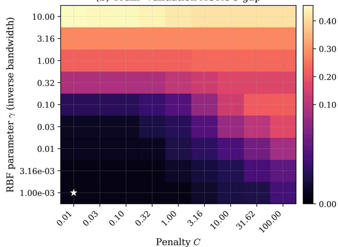
(b) Train--validation AUROC gap
